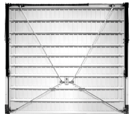
Above: SBD (Secured by Design) Garador Carlton Canopy Up-and-Over Garage Door with 4 point locking
